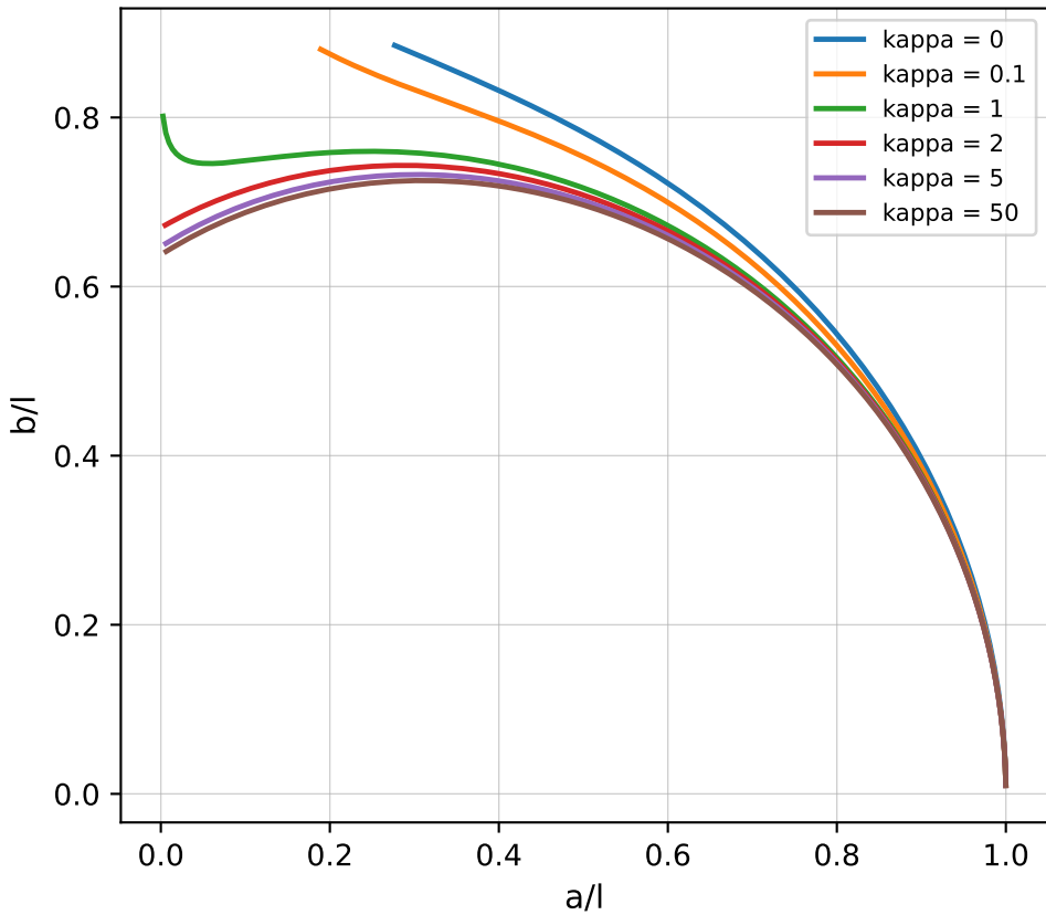
Continuous Beam Tip Loci for Varying Load Ratio
